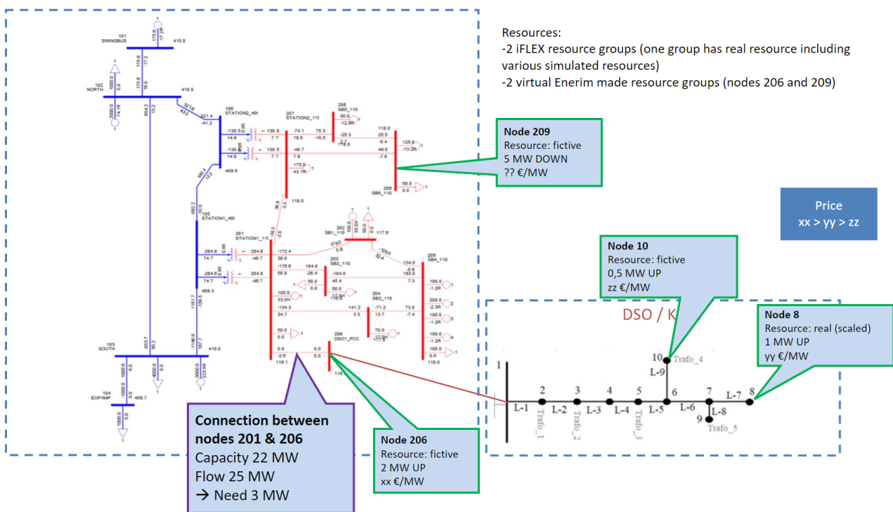
Figure 5-1: Scenario of the iFLEX-OneNet demonstration.
