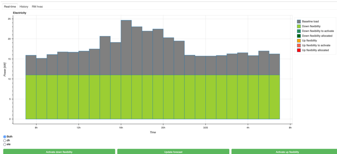
Figure 5-3. Schedule forecast of iFLEX building before flexibility activation.
