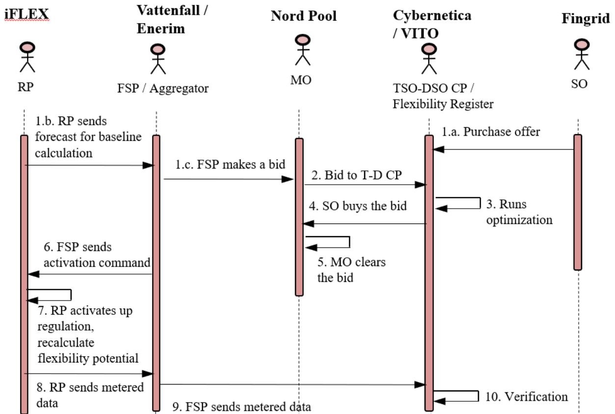
Figure 5-2: Process flow of the iFLEX-OneNet demonstration.
